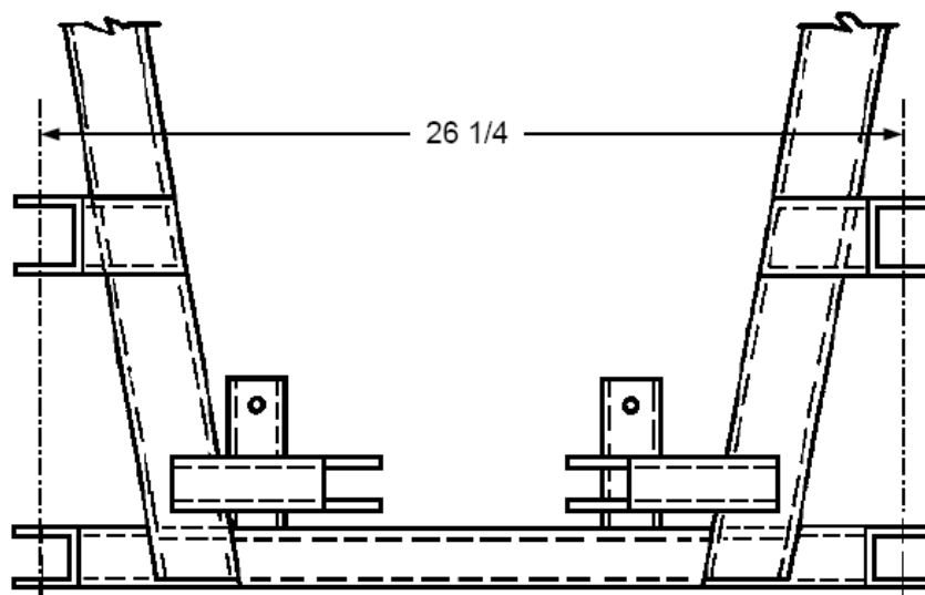
Figure 3- Position Rear Adjusters
