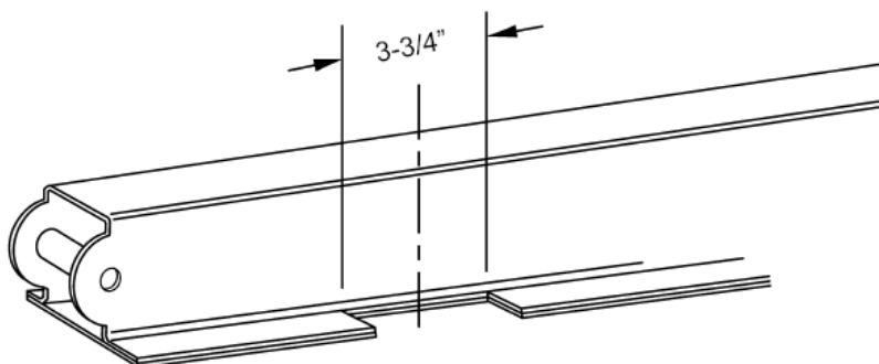
Figure 3- Trim Outer Flange
