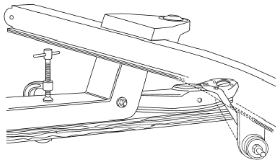
Figure 7- Strut Rod Install
