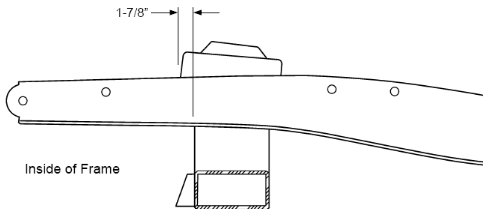
Figure 5- Spring Tower Install
