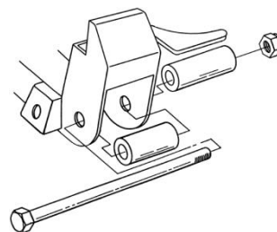
Figure 2- Crossmember Spacers Install
