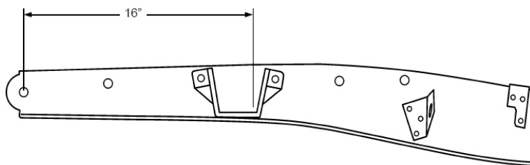
Figure 1- Spindle Centerline
