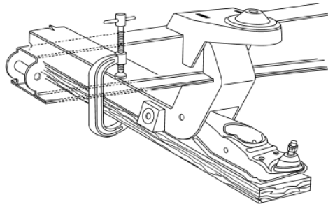
Figure 6- Lower Control Arm Install
