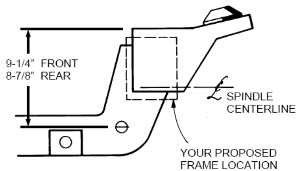
Figure 1- Setting Ride Height
