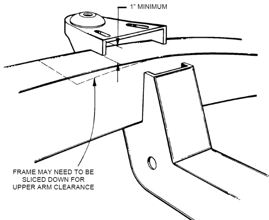
Figure 6- Spring Tower Trim To Fit
