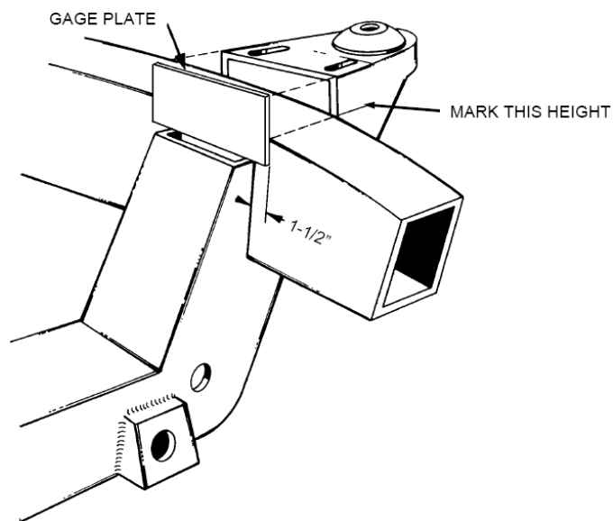
Figure 4- Spring Tower Install
