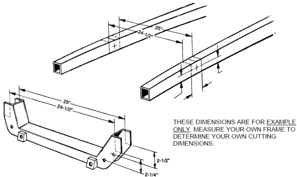
Figure 3- Crossmember Dimensions
