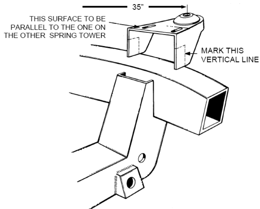
Figure 5- Spring Tower Install
