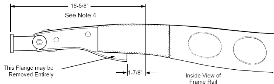
Figure 1- Boxing Plates Install & Trim Flange
