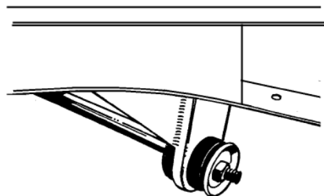
Figure 7- Strut Rod Install
