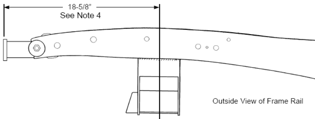
Figure 3- Crossmember Install
