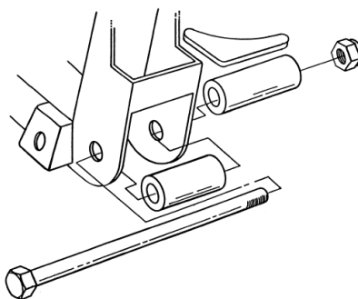
Figure 2- Mount Crossmember Spacers
