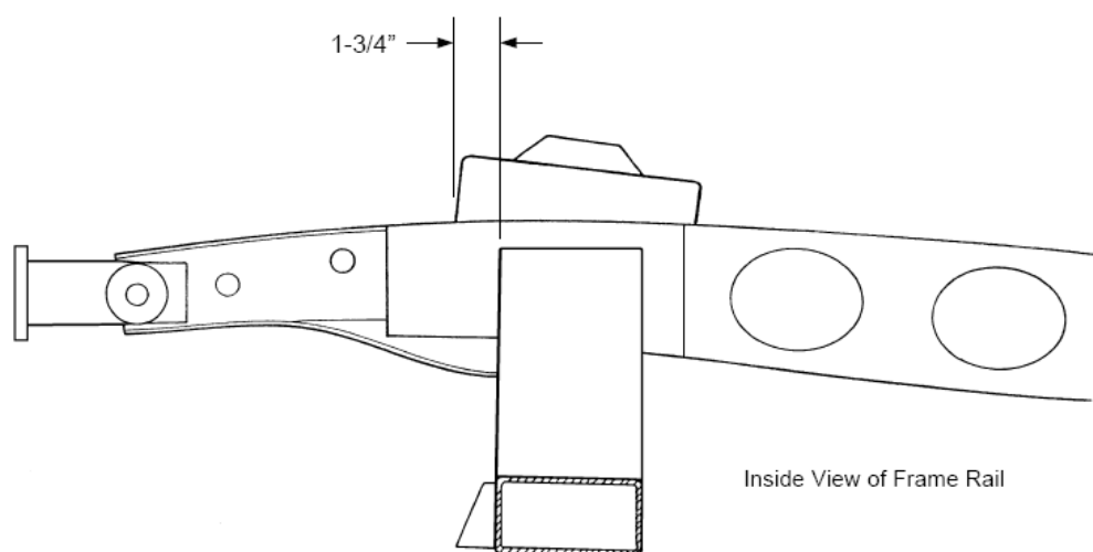
Figure 4- Spring Tower Install
