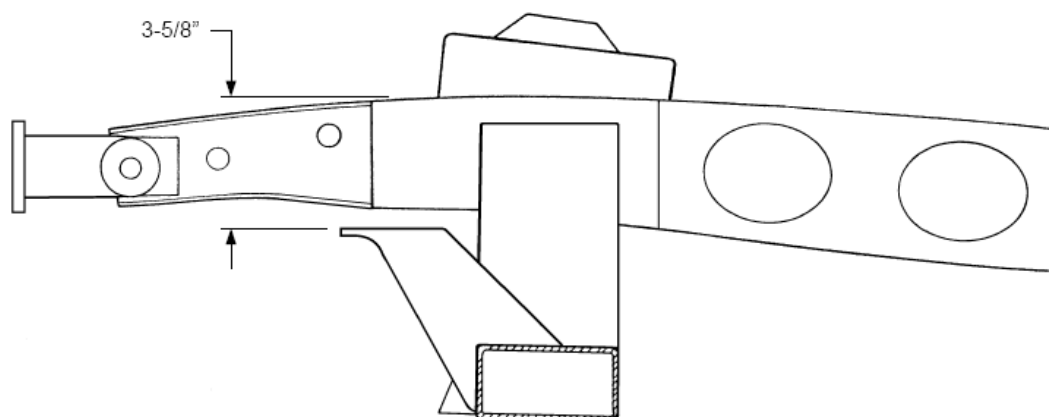
Figure 5- Radiator Support Install
